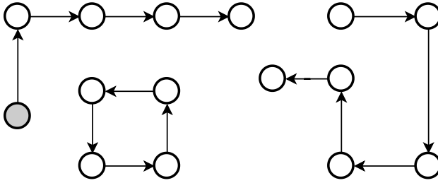
Figure 4.7: Any instance of END-OF-LINE consists of a set of paths and cycles, such as the instance shown here. Given the Parent / Child functions and a source node (a node with no parent node; here shaded in gray), is there an efficient polynomial-time algorithm to find a sink node (a node with no child node) or a different source node?
