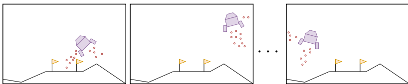
Figure 8.2: An illustration of the correlations of consecutive experiences in an environment where the agent controls a spaceship to land. In the first two episodes, the agent approaches the goal location from the right side. In the third episode, the agent has to approach the goal location from the left side and, thus, experiences very different states than in the previous episodes.
