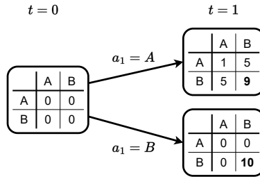
Figure 9.13: Two-step common-reward stochastic game with three states. The transition function across the three states and the reward function within each state is shown here. In the initial state the agents receive no rewards for any action and agent 1 decides which matrix game to choose in the next time step: either the linearly decomposable game, as represented by the state in the top right, or the monotonically decomposable game, as represented by the state in the bottom right.
