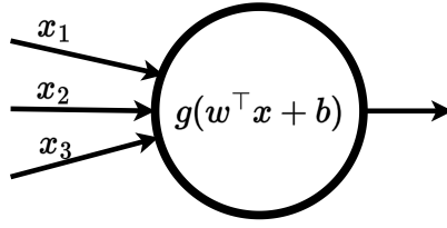
Figure 7.3: An illustration of a single neural unit computing a scalar output given an input x \in \mathbb{R}^3 . First, a weighted sum over the input features is computed using the vector multiplication of w \in \mathbb{R}^3 and the input x and a scalar bias b \in \mathbb{R} is added. Finally, a non-linear activation function g : \mathbb{R} \rightarrow \mathbb{R} is applied to obtain the scalar output.
