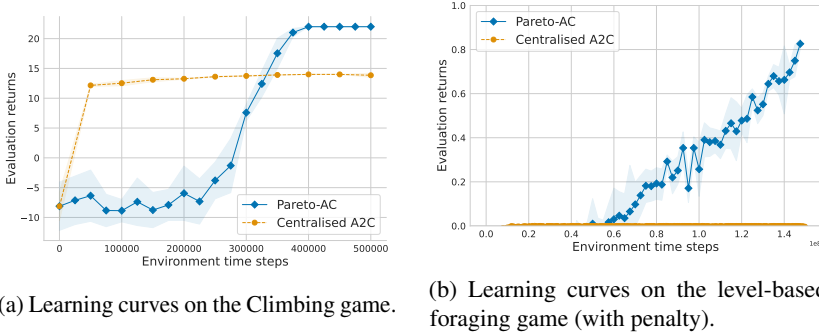
Figure 9.6: Learning curves comparing centralized A2C with Pareto-AC in the Climbing and level-based foraging games.
